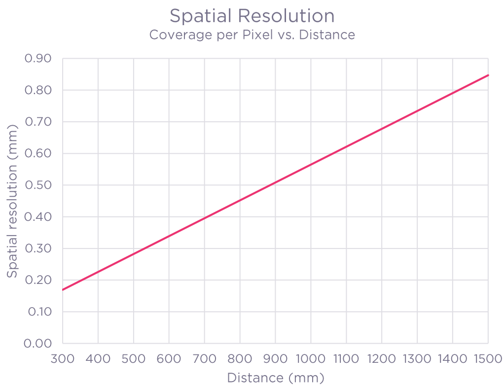
FIGURE 3 – SPATIAL RESOLUTION
