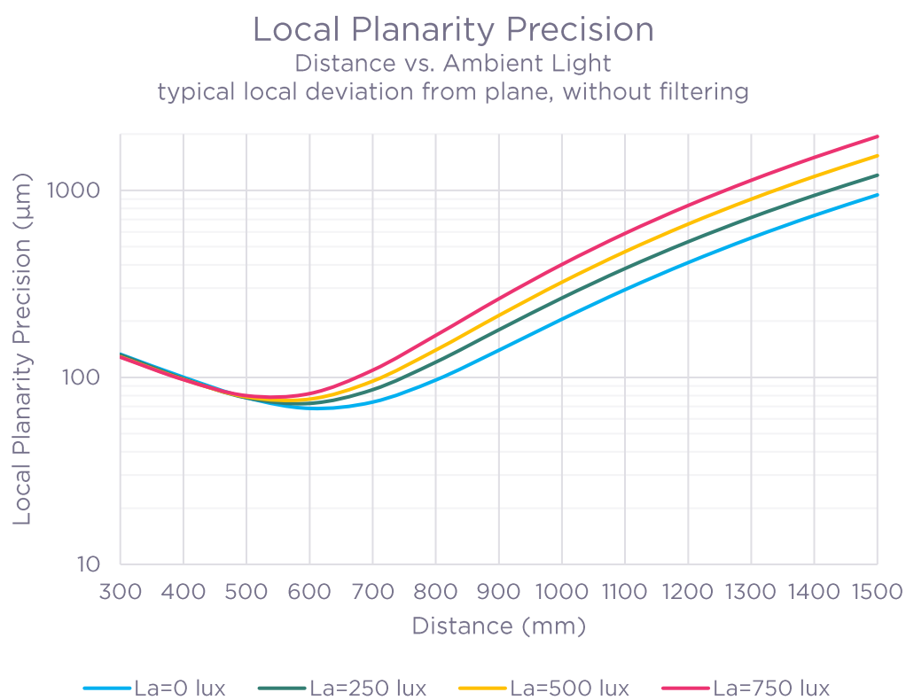
FIGURE 9 - LOCAL PLANARITY PRECISION VS. DISTANCE
